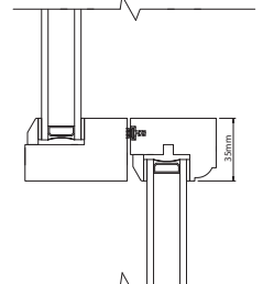
04: BOX HEAD SCALE 1:5
