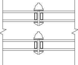
01: GLAZING BAR SCALE 1:5
