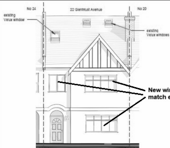
1 Proposed Front Elevation 1 : 100
