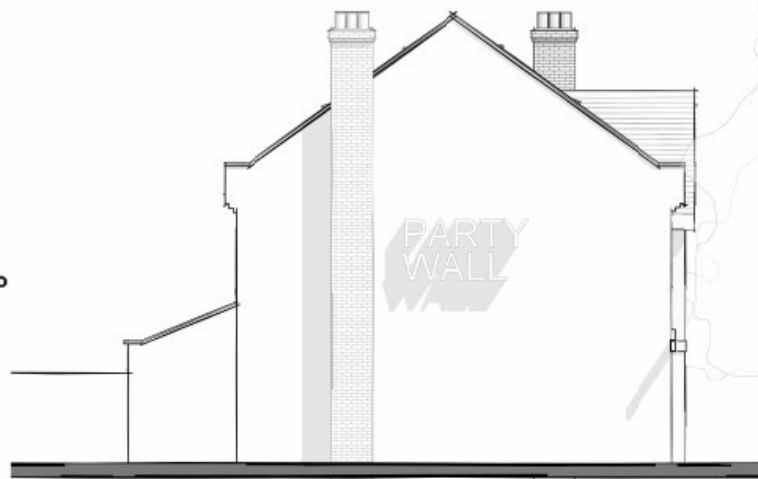
2 Proposed West Elevation 1 : 100
