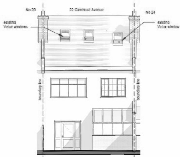
3 Existing Rear Elevation 1 : 100
