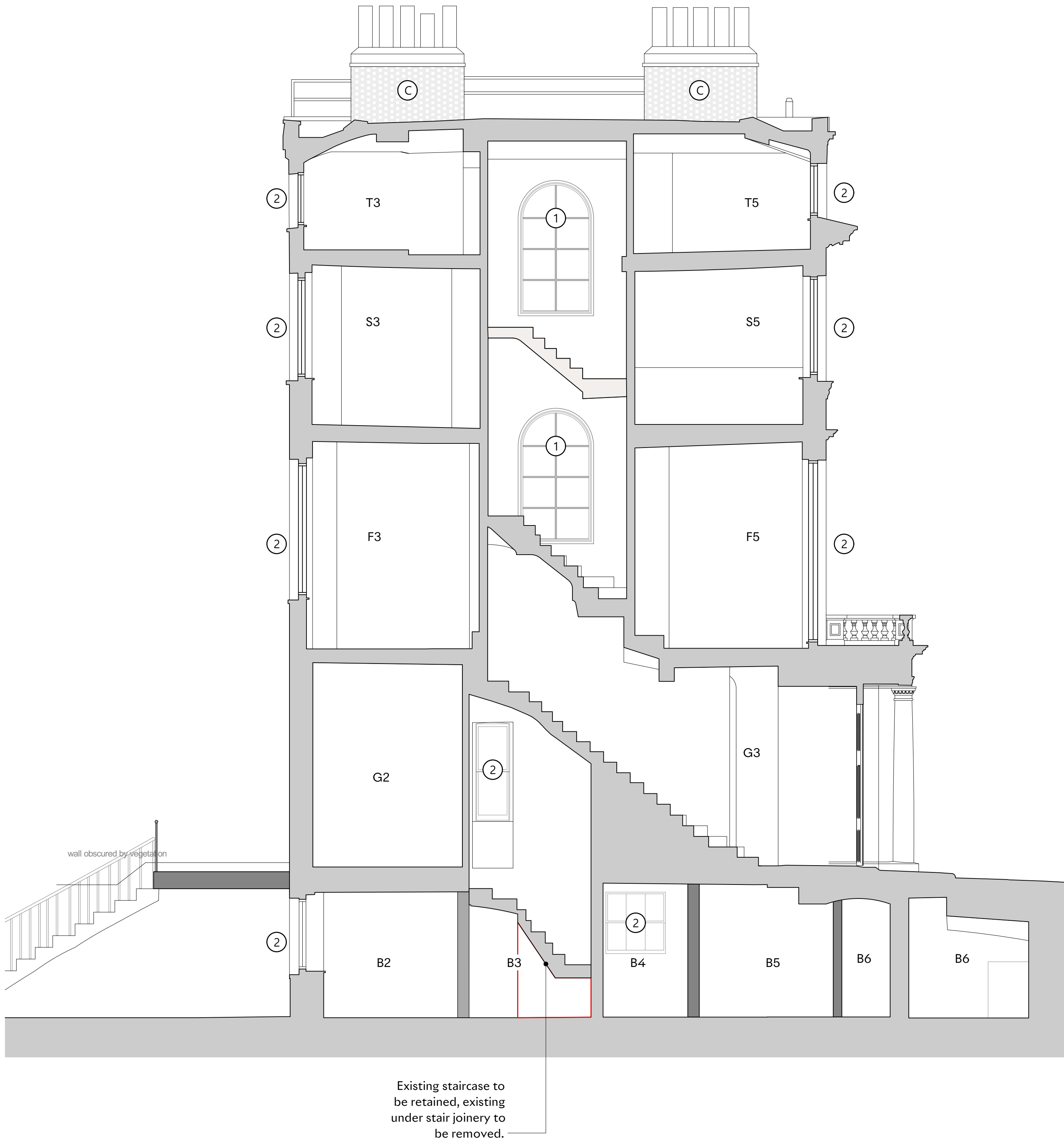
1 Proposed Section A-A Scale: 1:50
