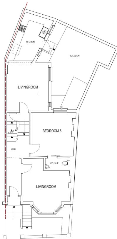
2 PLAN - GROUND FLOOR EXISTING 1:100
